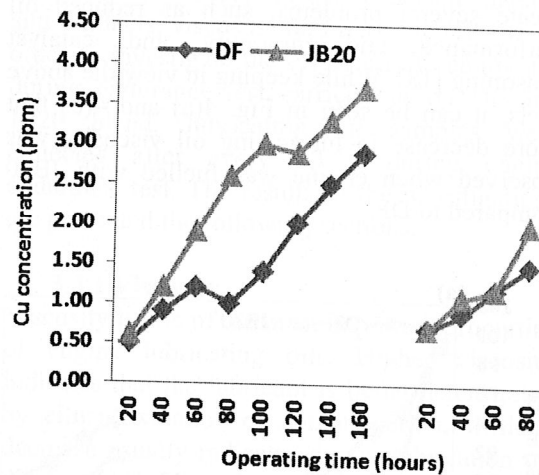
Fig. 8 Cu concentration vs. engine running time
