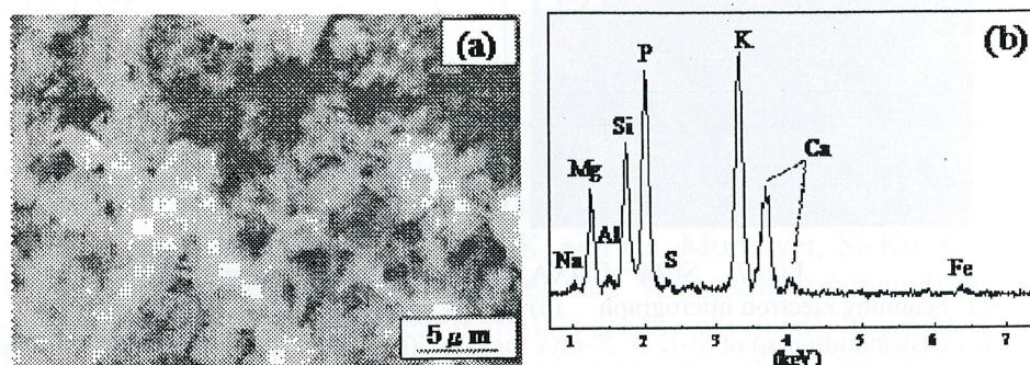
Fig. 9. SEM-EDXA on ash from the Kernel Cake.
