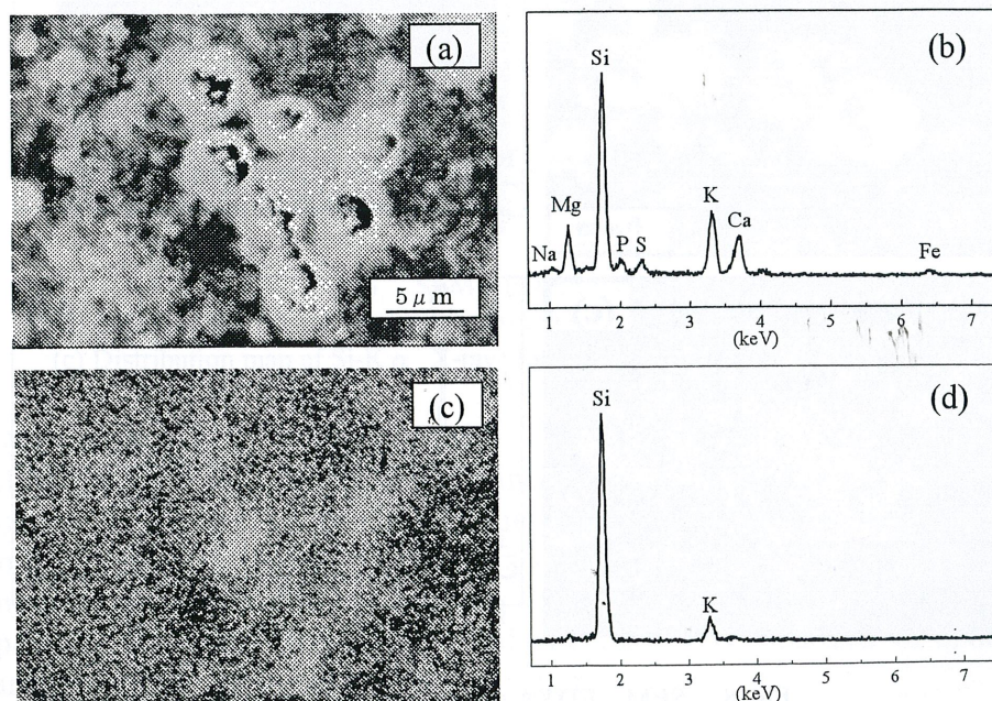
Fig. 10. SEM-EDXA on ash from the EFB.
